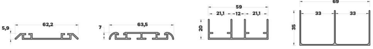
MB-5050 (0,309 kg/mt) ALT RAY PROFİLİ
