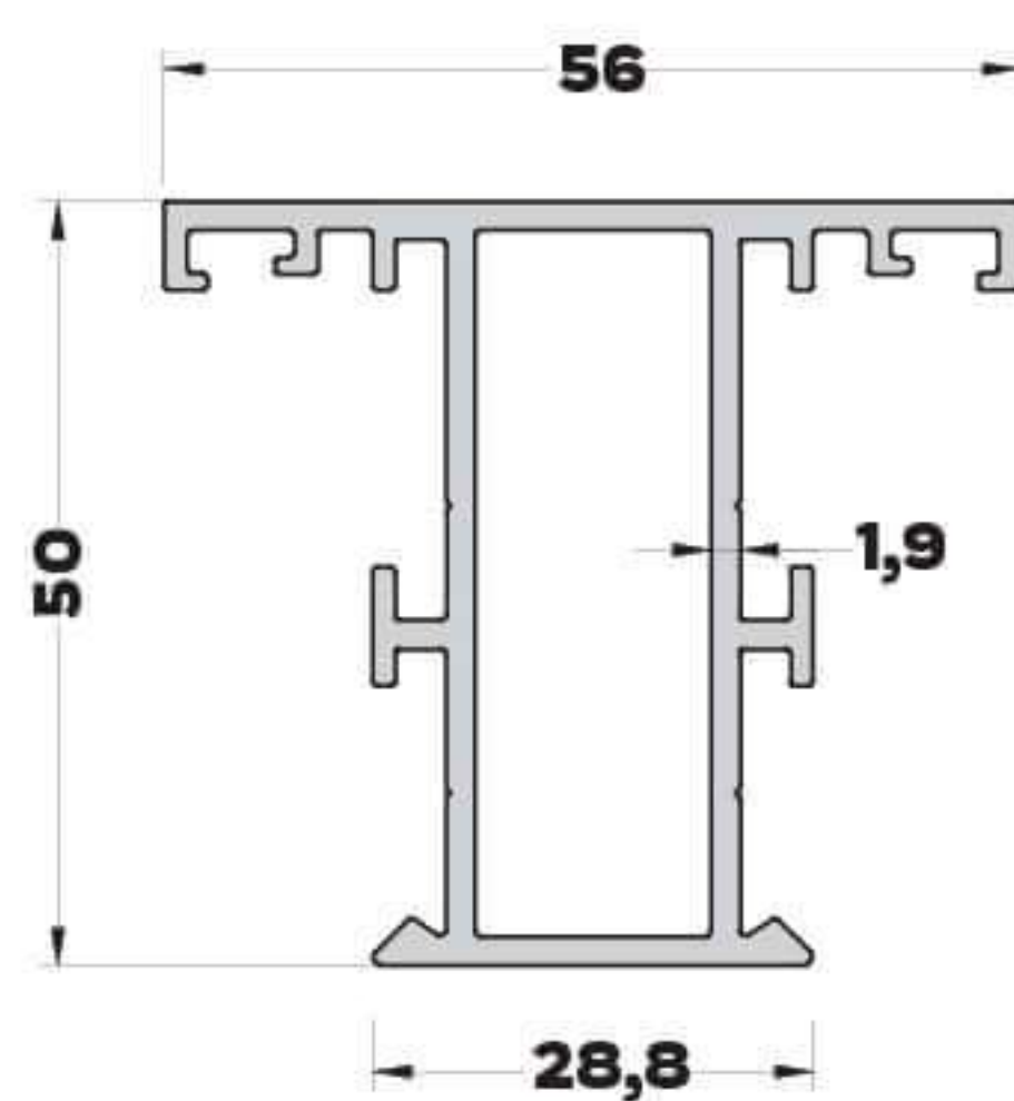
AB-6542 (1,125 kg/mt) ORTA KAYIT PROFİLİ
