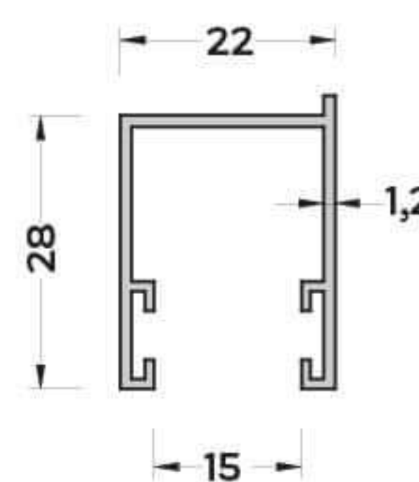
P-4062 (1,215 kg/mt) PANJUR YAN KASA PROFİLİ
