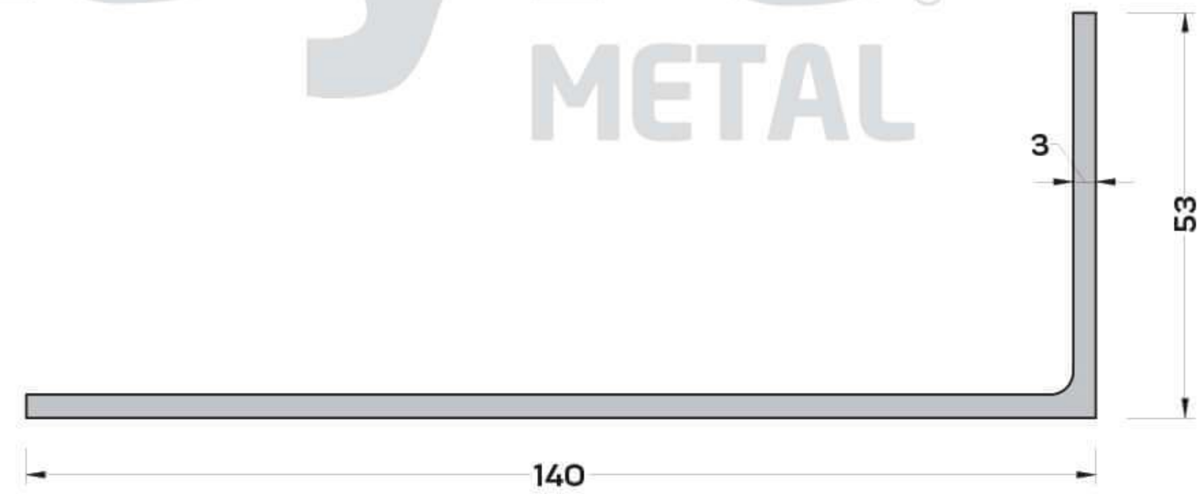
CK-4295 (1,549 kg/mt) L ANKRAJ PROFİLİ
