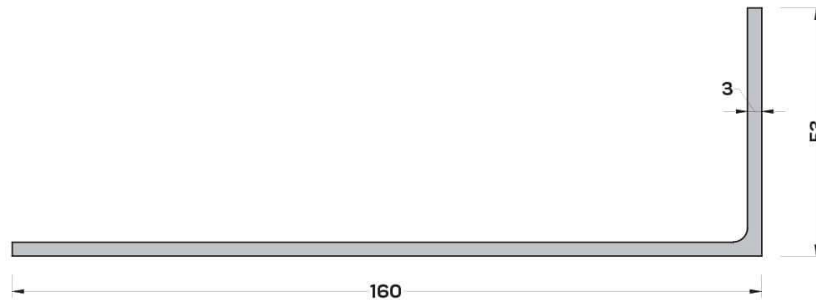
CK-4293 (1,712 kg/mt) L ANKRAJ PROFİLİ
