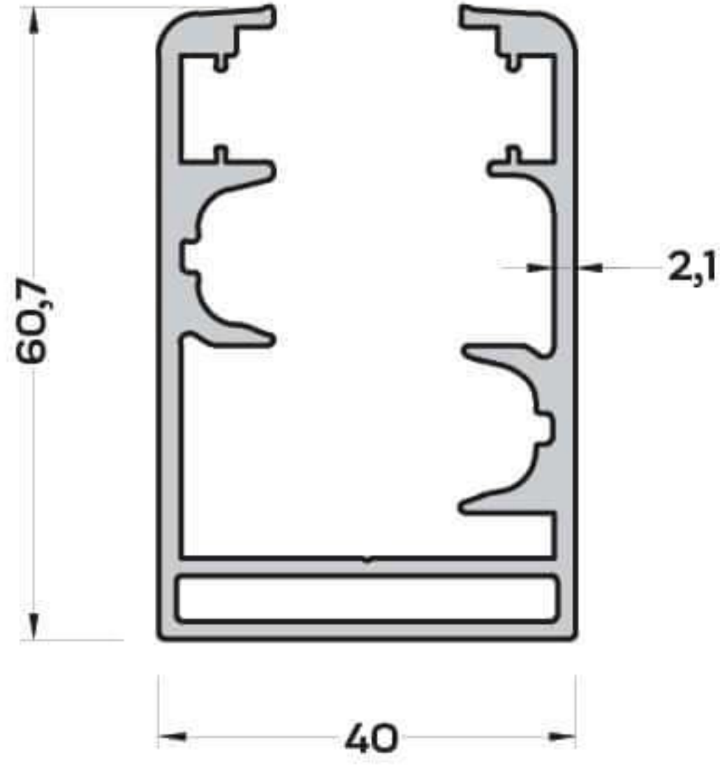
900-1101 (1,475 kg/mt) GOLD KASA PROFİLİ
