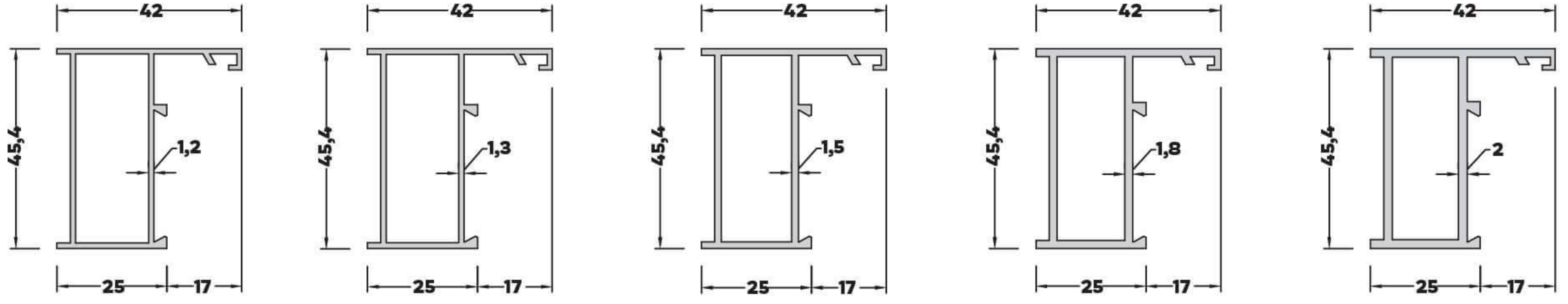
AL-3080 (0,548 kg/mt) DAR KASA PROFİLİ
