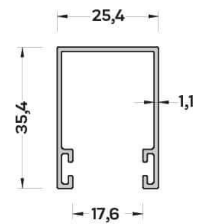
P-8482 (1,315 kg/mt) PANJUR YAN KASA PROFİLİ
