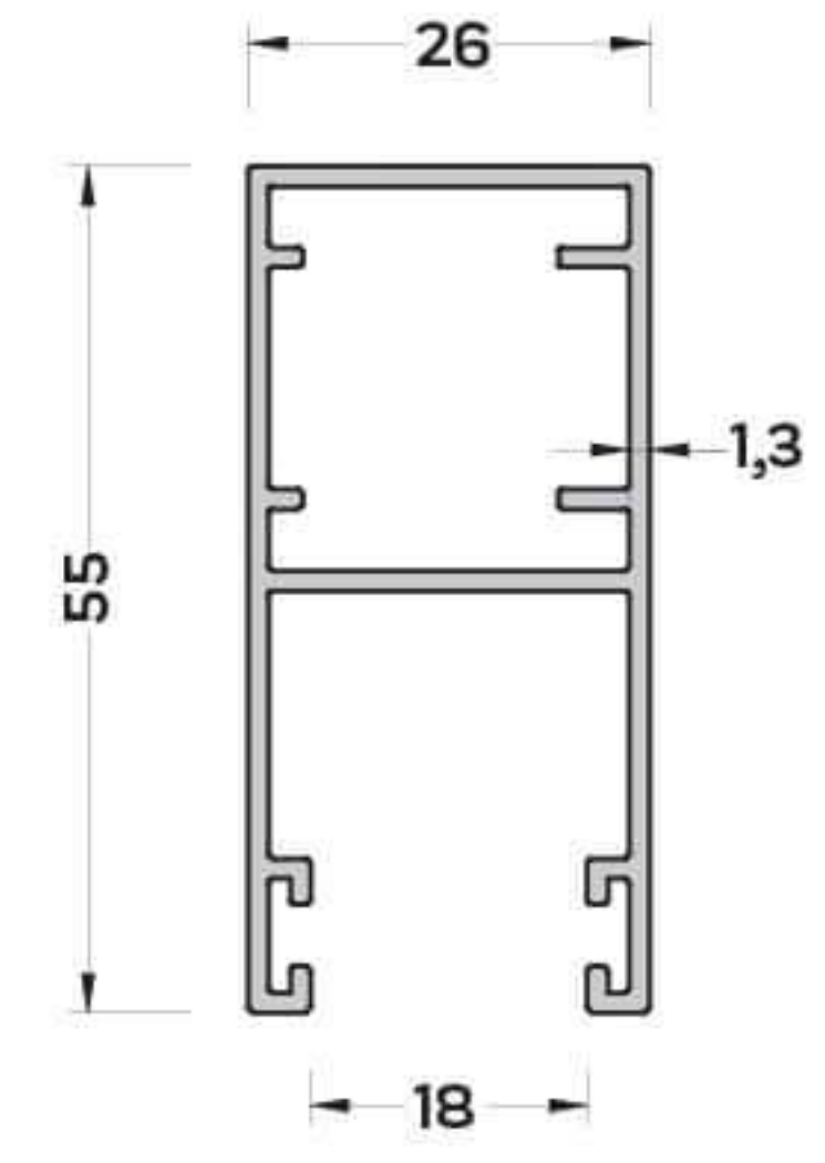
P-3457 (0,662 kg/mt) PANJUR YAN KASA PROFİLİ
