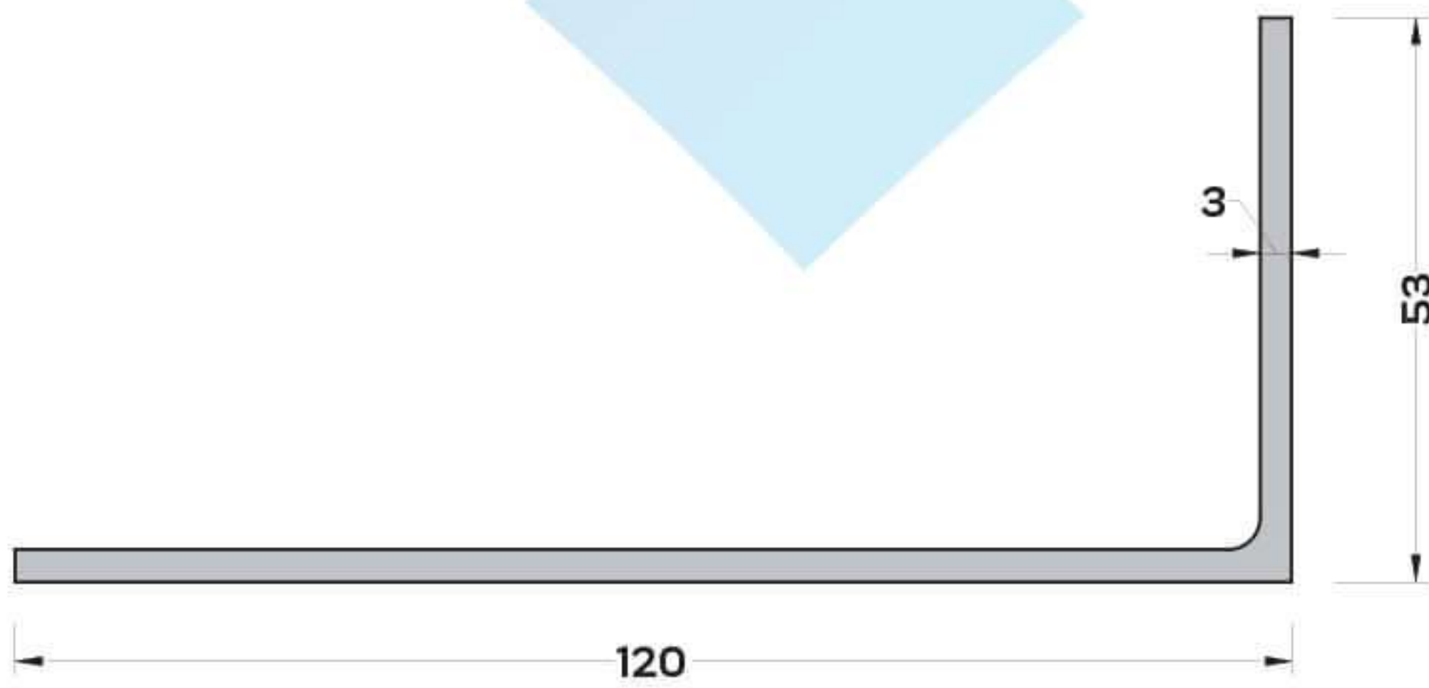
CK-4294 (1,387 kg/mt) L ANKRAJ PROFİLİ
