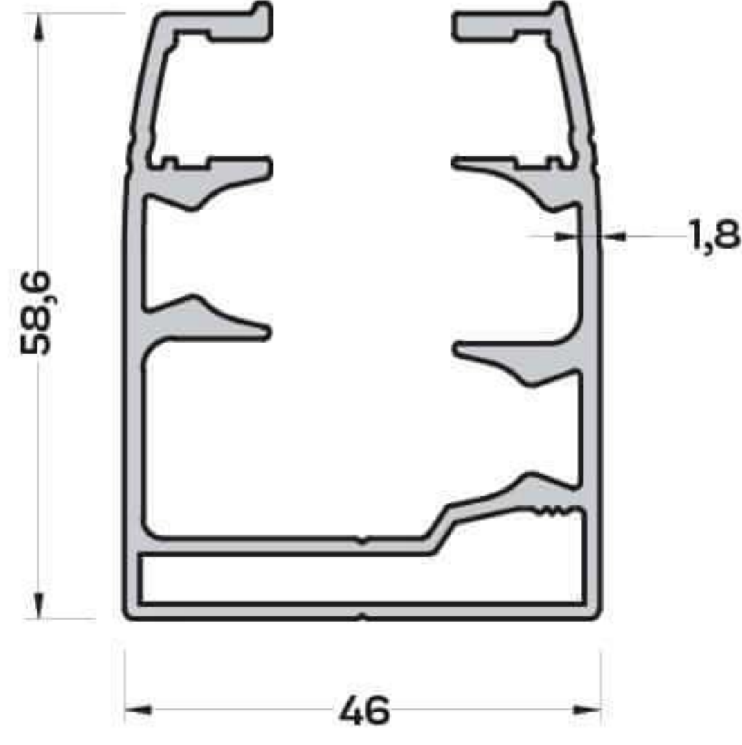
900-1102 (1,436 kg/mt) FIRTINA KASA PROFİLİ
