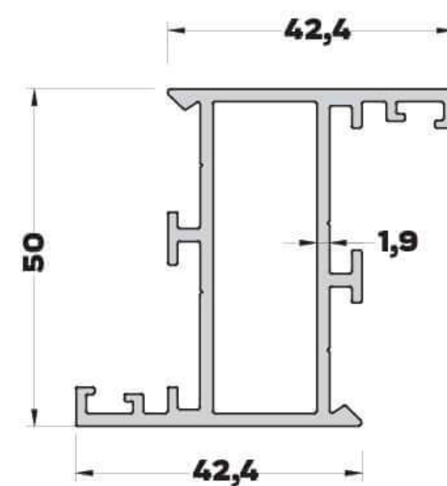
AB-6544 (1,125 kg/mt) Z KASA PROFİLİ
