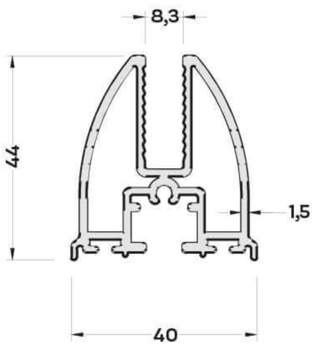
900-1101 (1,475 kg/mt) GOLD KASA PROFİLİ
