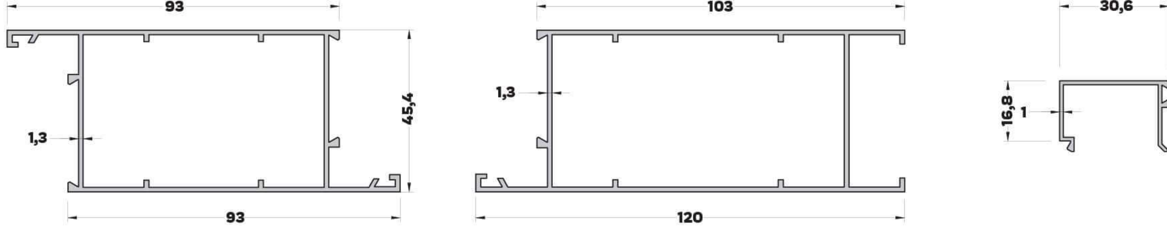
AL-3045 (1,088 kg/mt) KAPI KANAT PROFİLİ
