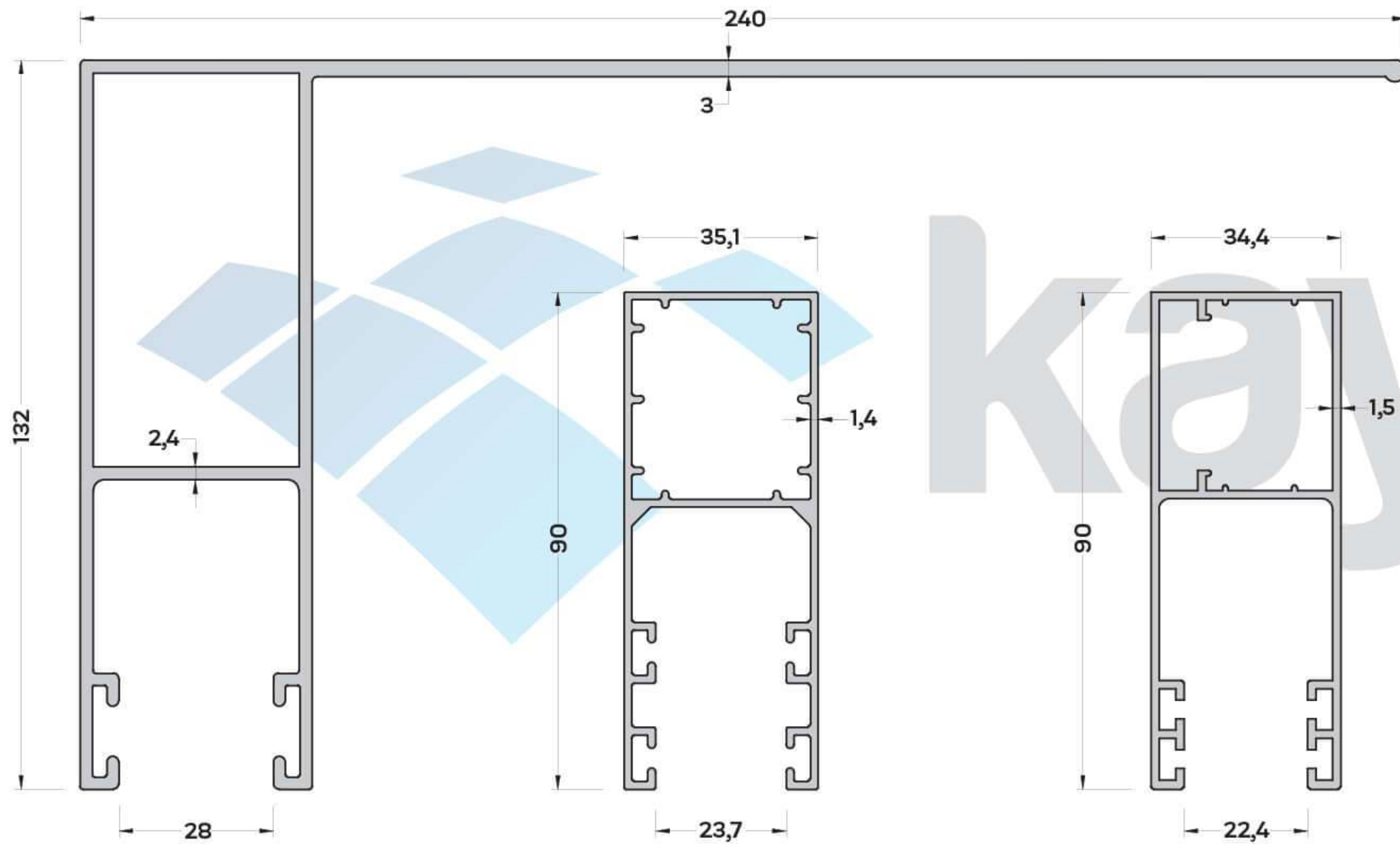
P-3947 (0,560 kg/mt) PANJUR YAN KASA PROFİLİ
