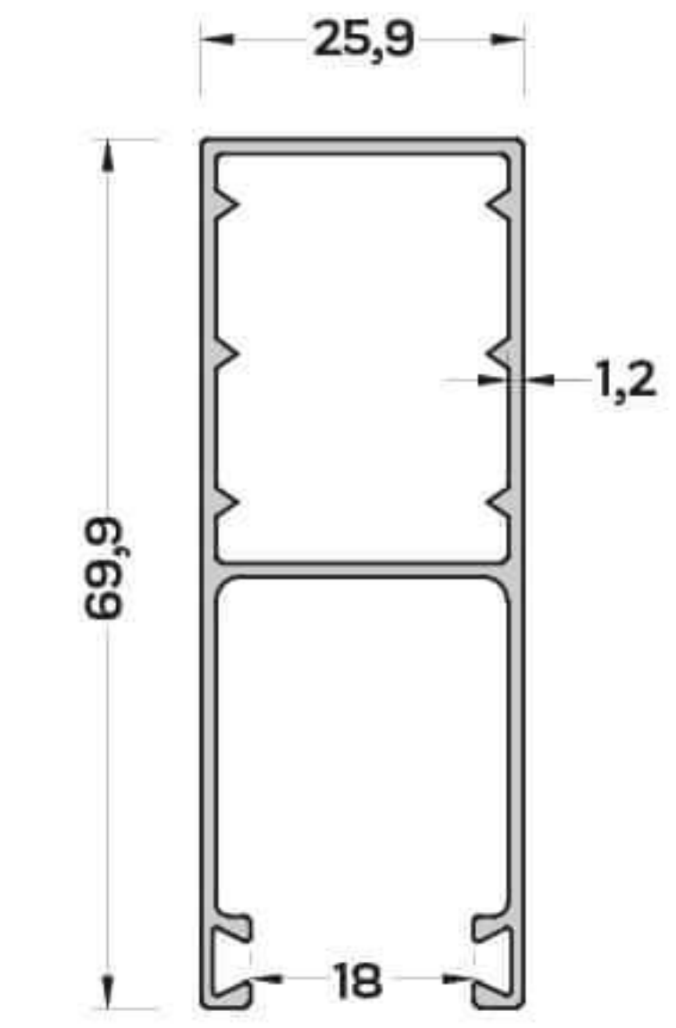
P-3457 (0,662 kg/mt) PANJUR YAN KASA PROFİLİ
