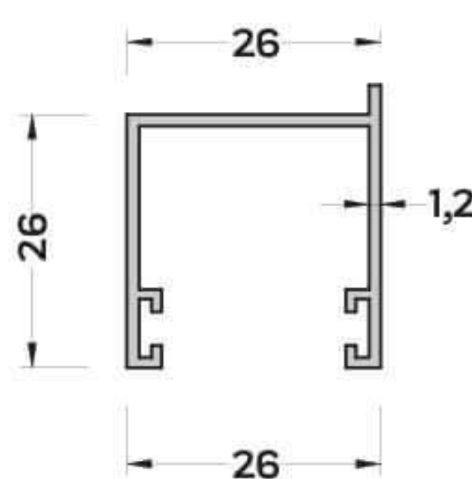
P-5040 (1,220 kg/mt) PANJUR YAN KASA PROFİLİ
