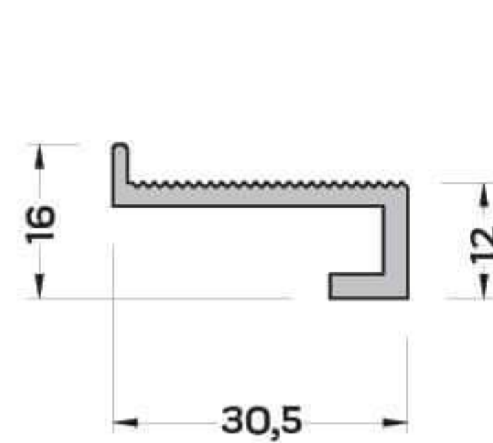
CK-6750 (0,328 kg/mt) ALT ASKI PROFİLİ
