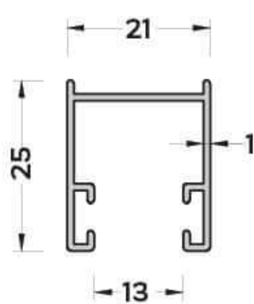
P-3416 (3,994 kg/mt) PANJUR YAN KASA PROFİLİ
