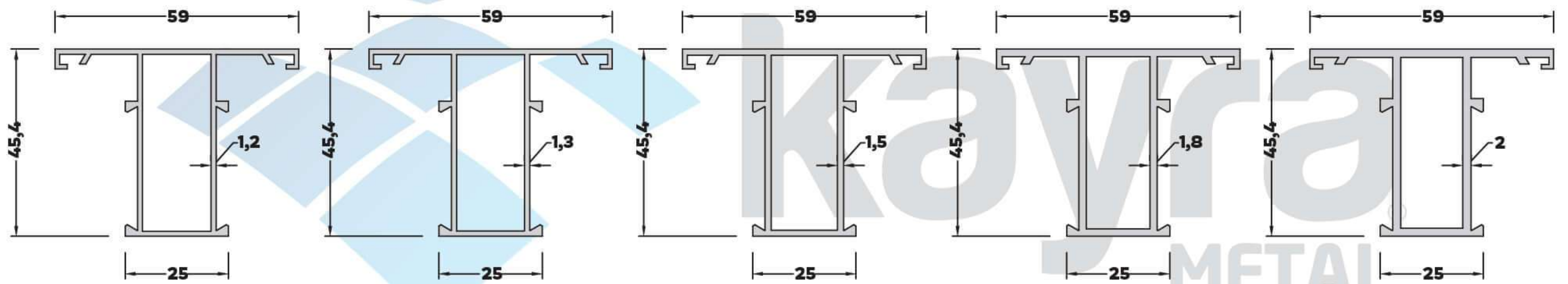
AL-3073 (0,548 kg/mt) GENİŞ KASA PROFİLİ
